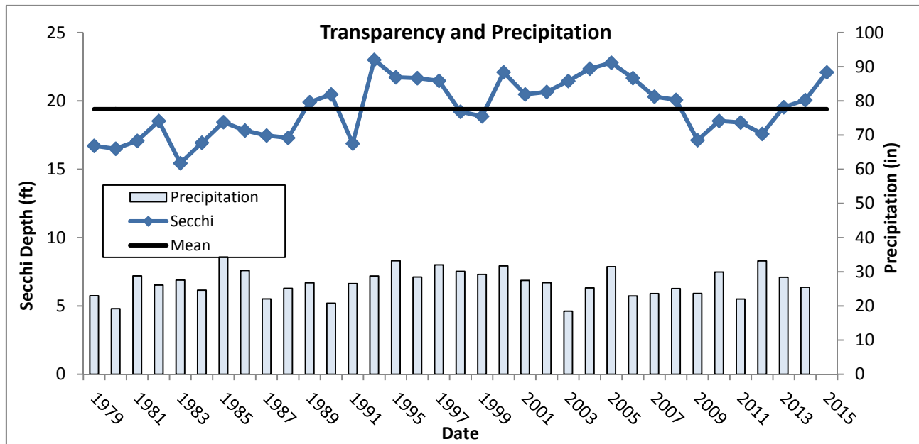
Figure 3. Annual mean transparency compared to long-term mean transparency at the Main Bay site 202.
