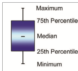
Legend for Figure 19 below.
