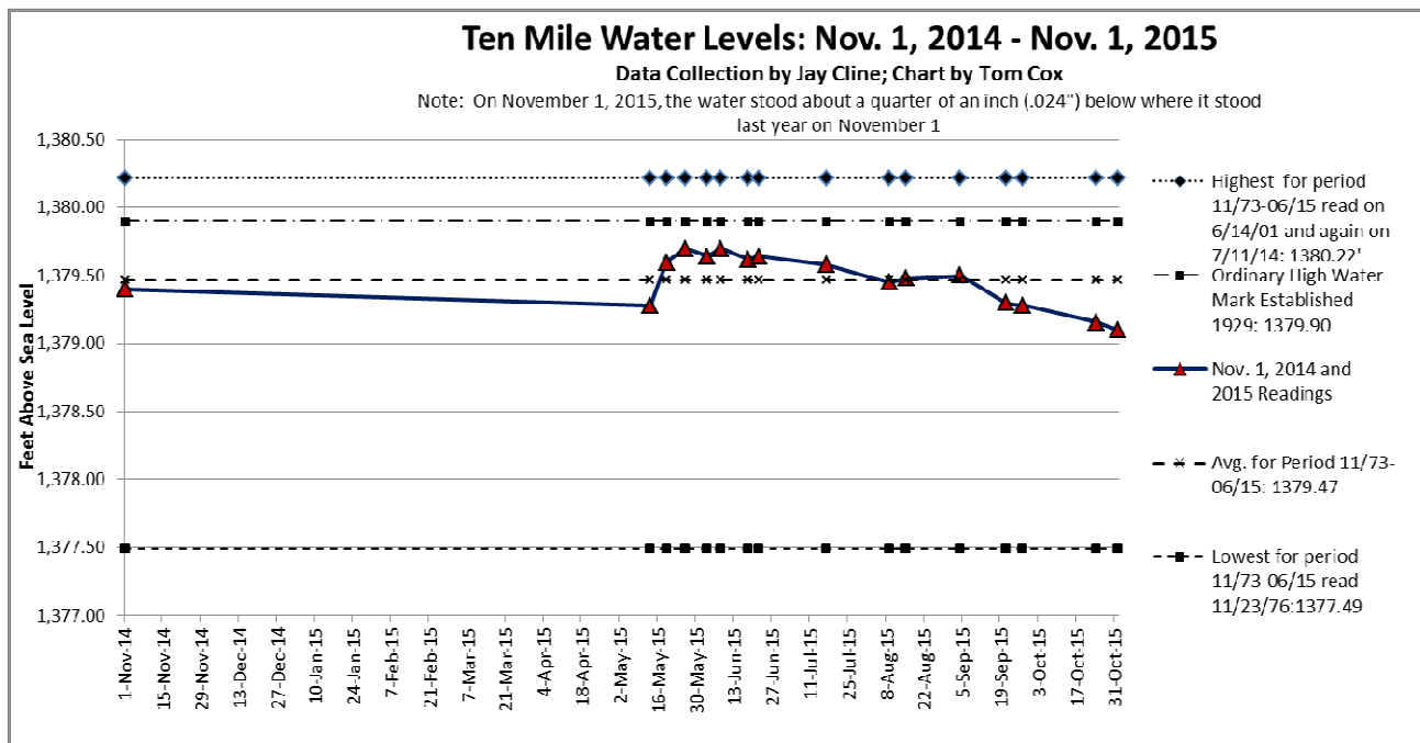
Figure 25. Ten Mile Lake water levels, 2015, Ten Mile Lake Association.
