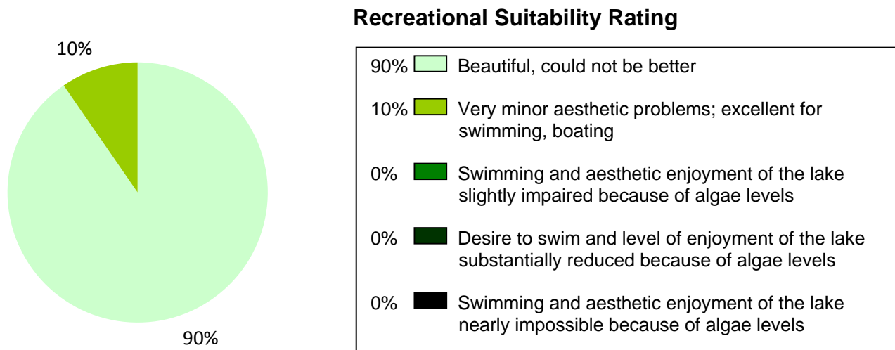
Figure 7. Recreational suitability rating, as rated by the volunteer monitor.
