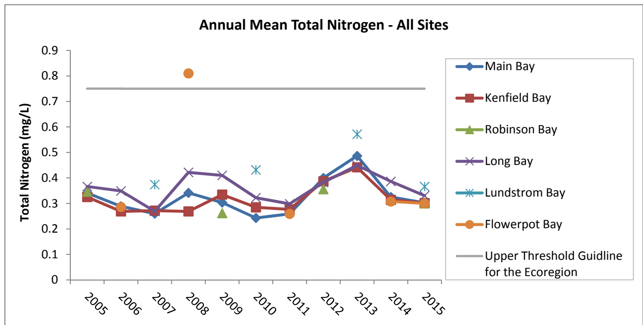
Figure 12. Historical annual mean total nitrogen concentrations (ug/L) for Ten Mile Lake comparing sites.
