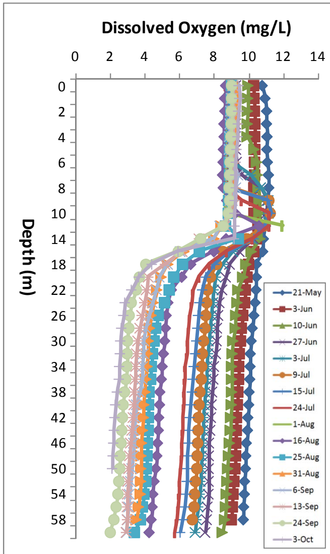
Figure 13. Dissolved oxygen profile for Ten Mile Lake in 2015. mg/L in the hypolimnion for most of the cold water fish species such as Cisco Lake is considered a Tier 1 Cisco refuge require cold, oxygenated water to survive and the loss of Ciscos can indicate eutrophication in lakes. Ten Mile Lake also supports a lake whitefish population, which also requires cold, well-oxygenated water (Figure 14).
