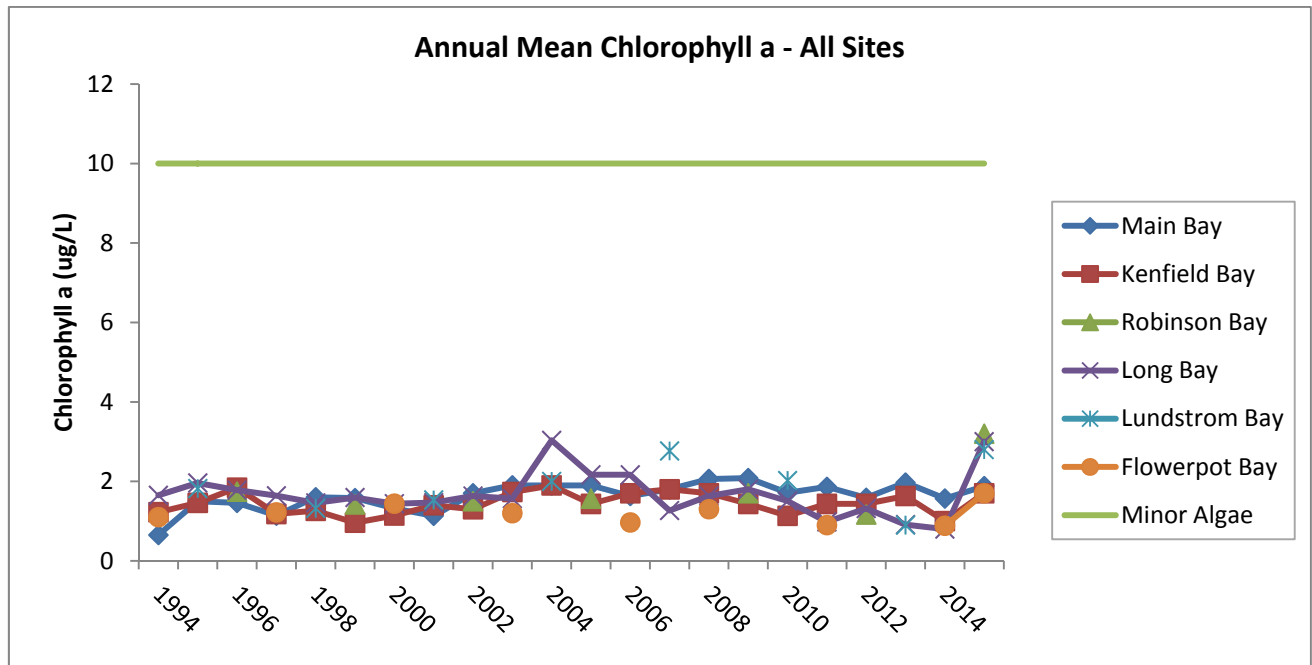
Figure 11. Historical annual mean chlorophyll a concentrations (ug/L) for Ten Mile Lake comparing sites.
