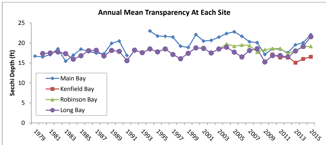
Figure 4. Annual mean transparency comparison between sites.
