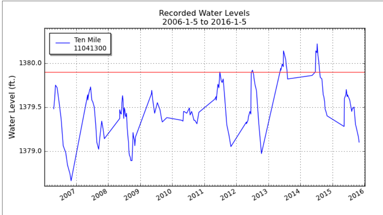
Figure 24. Ten Mile Lake water levels from 2006-2015, MN DNR.
