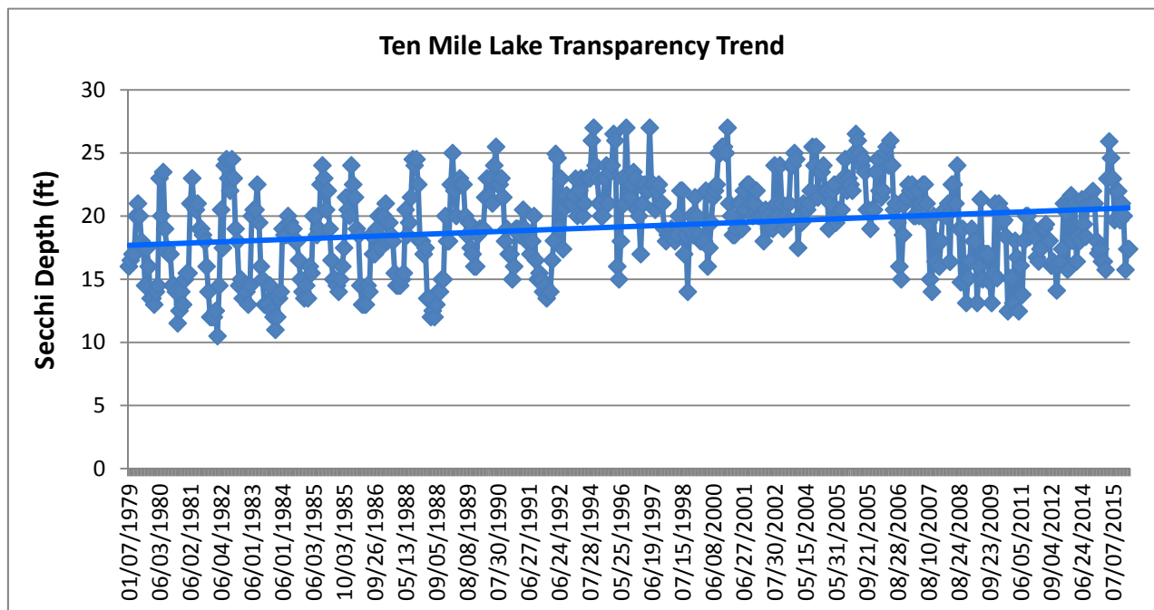
Figure 17. Transparency (feet) trend for site 202 from 1979-2015.
