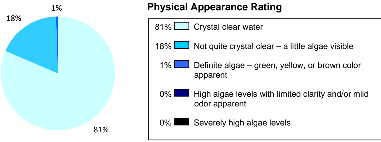
Figure 6. Ten Mile Lake physical appearance ratings by samplers.
