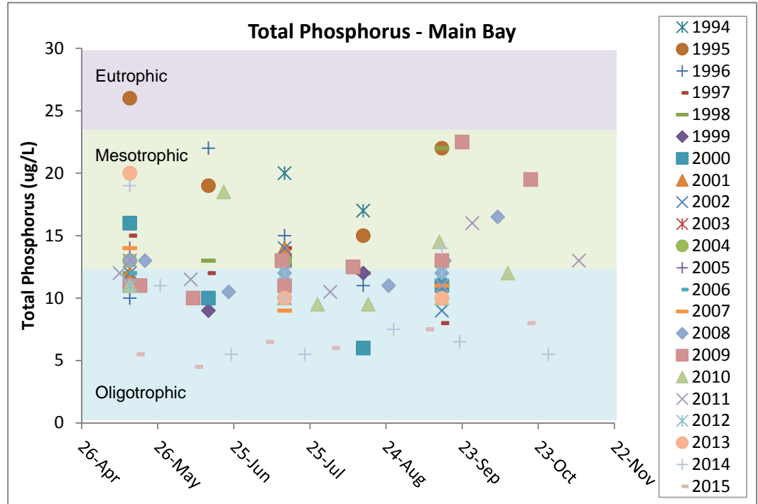
Figure 8. Historical total phosphorus concentrations (ug/L) for Ten Mile Lake site 202.
