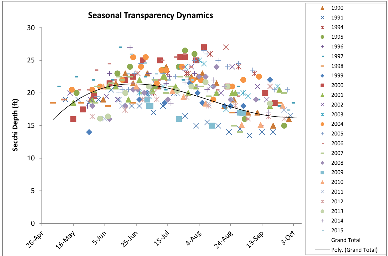
Figure 5. Seasonal transparency dynamics and year to year comparison (Primary Site 202). The black line represents the pattern in the data.
