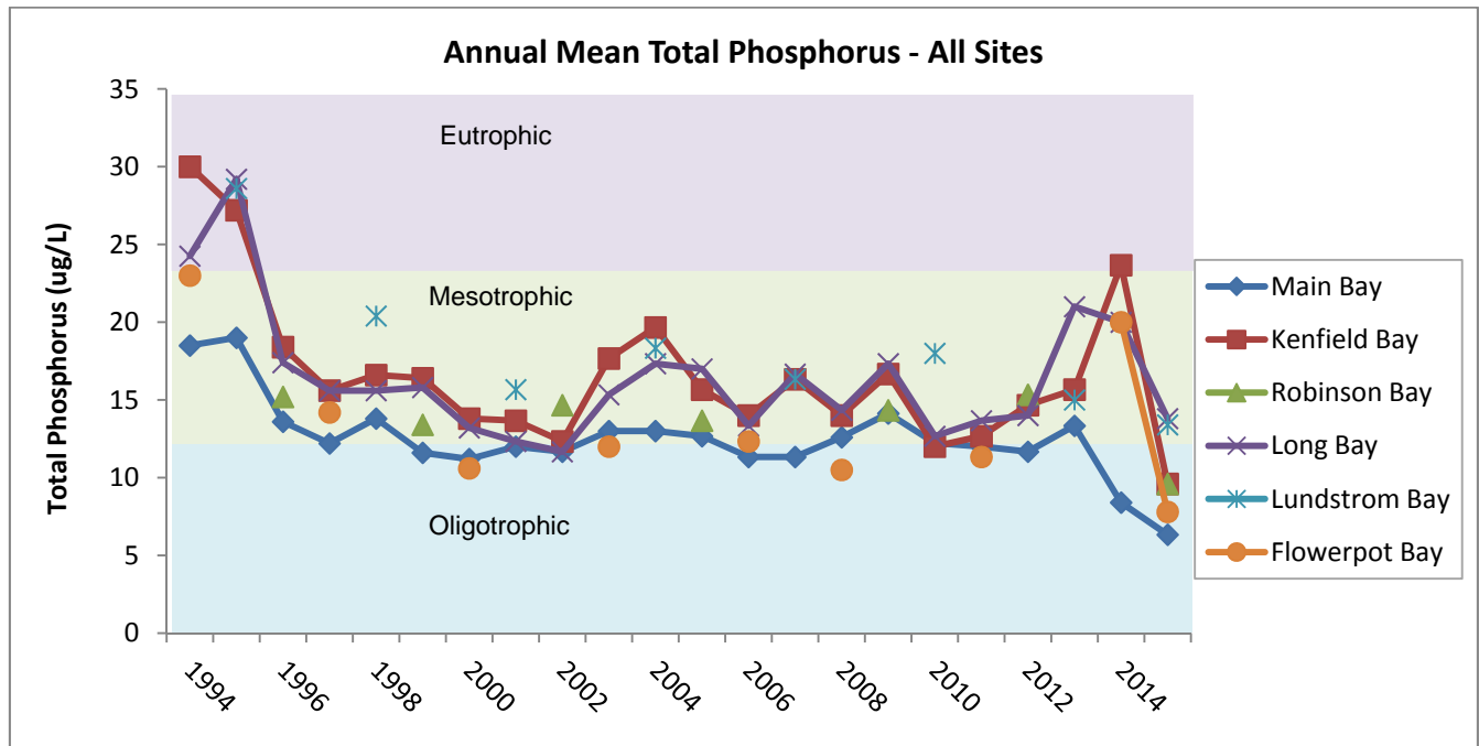
Figure 9. Historical annual mean total phosphorus concentrations (ug/L) for Ten Mile Lake comparing sites.
