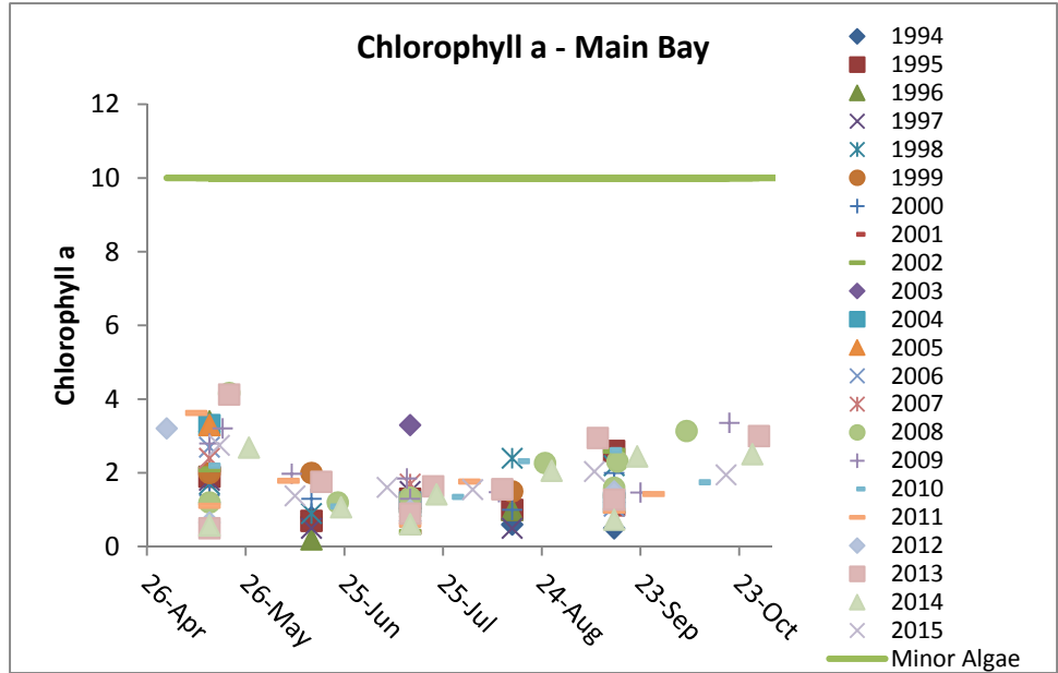
Figure 10. Chlorophyll a concentrations (ug/L) for Ten Mile Lake at site 202.
