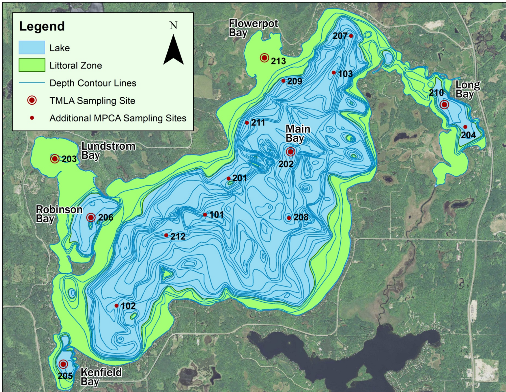
Figure 1. Map of Lake Name with 2010 aerial imagery and illustrations of lake depth contour lines, sample site locations, inlets and outlets, and public access points. The light green areas in the lake illustrate the littoral zone, where the sunlight can usually reach the lake bottom, allowing aquatic plants to grow.
