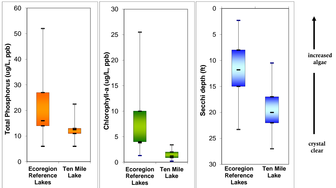
Figure 19. Ten Mile Lake (Main Basin) ranges compared to Northern Lakes and Forest Ecoregion ranges. The colored boxes represent the 25 th to 75 th percentile of the data for each the ecoregion reference lakes and Ten Mile Lake. The bars represent the maximum and the minimum. The Ten Mile Lake total phosphorus and chlorophyll a ranges are from 118 data points collected in May-September of 1994-2015. The Ten Mile Lake Secchi depth range is from 564 data points collected in May-September from 1979-2015.
